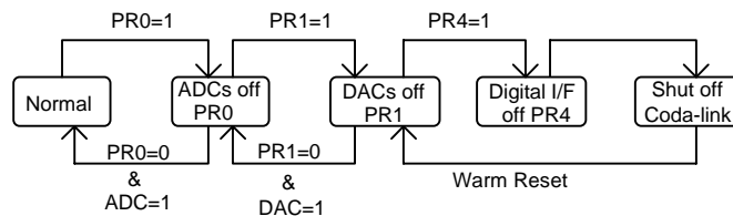
Figure 13. STAC9780/82 Powerdown/Powerup flow with analog still alive
