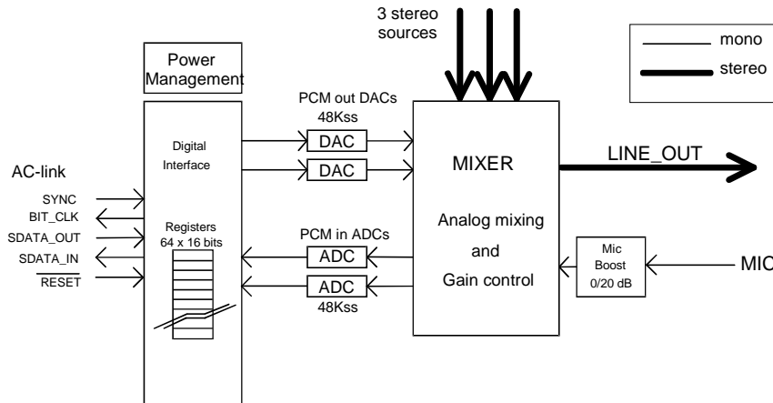
Figure 2. STAC9780/82 Block Diagram
