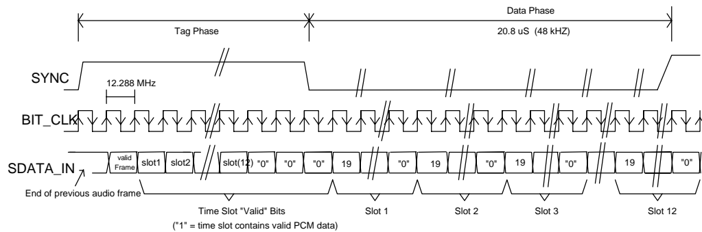
Figure 8. STAC9780/82 Audio Input Frame
