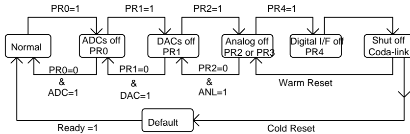
Figure 12. Example of STAC9780/82 Powerdown/Powerup flow
