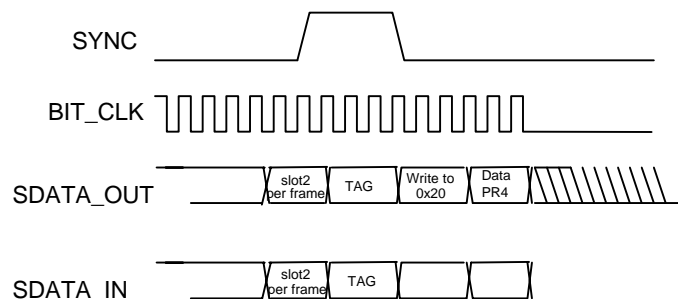
Figure 10. STAC9780/82 Powerdown Timing
